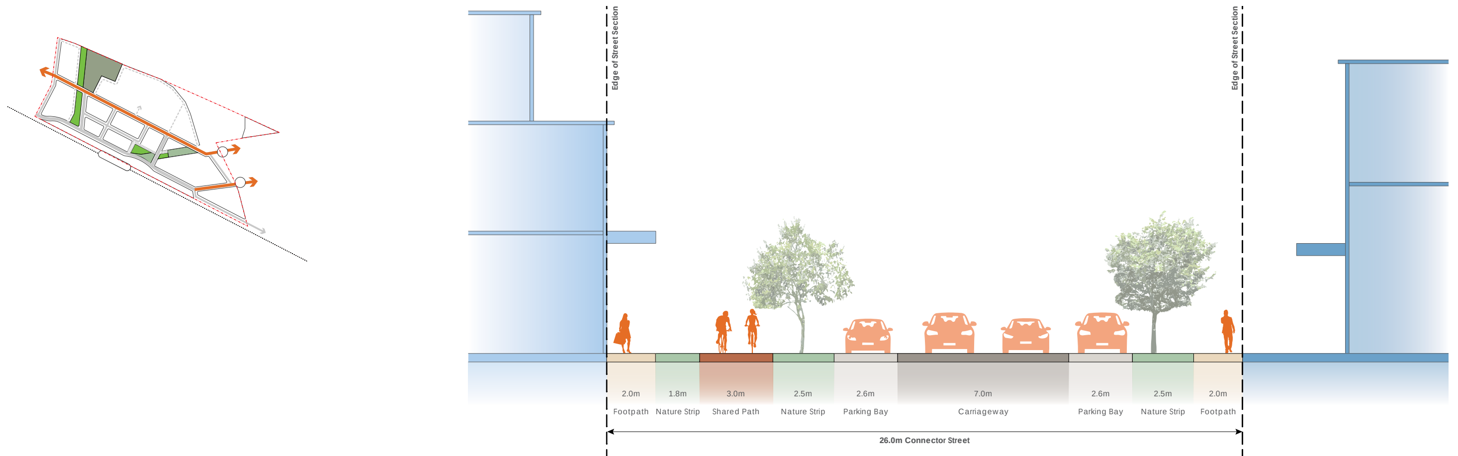
Figure 32 – Industrial Connector Street
